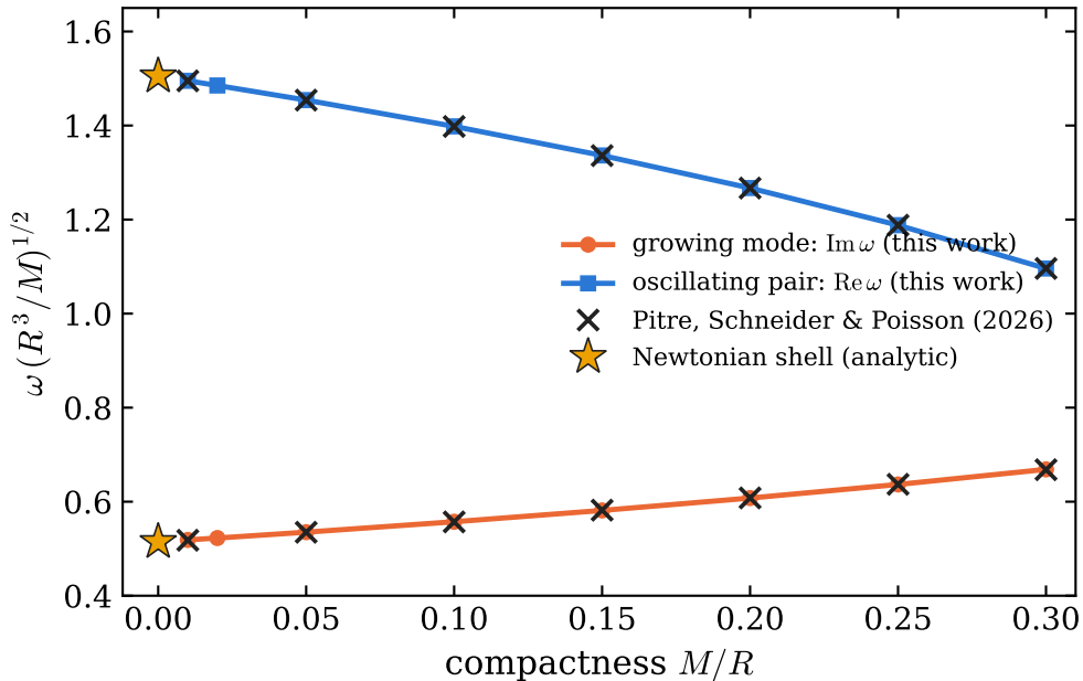
Even-parity matter modes of the static fluid shell ( \ell = 2 , \Gamma = 2 )
